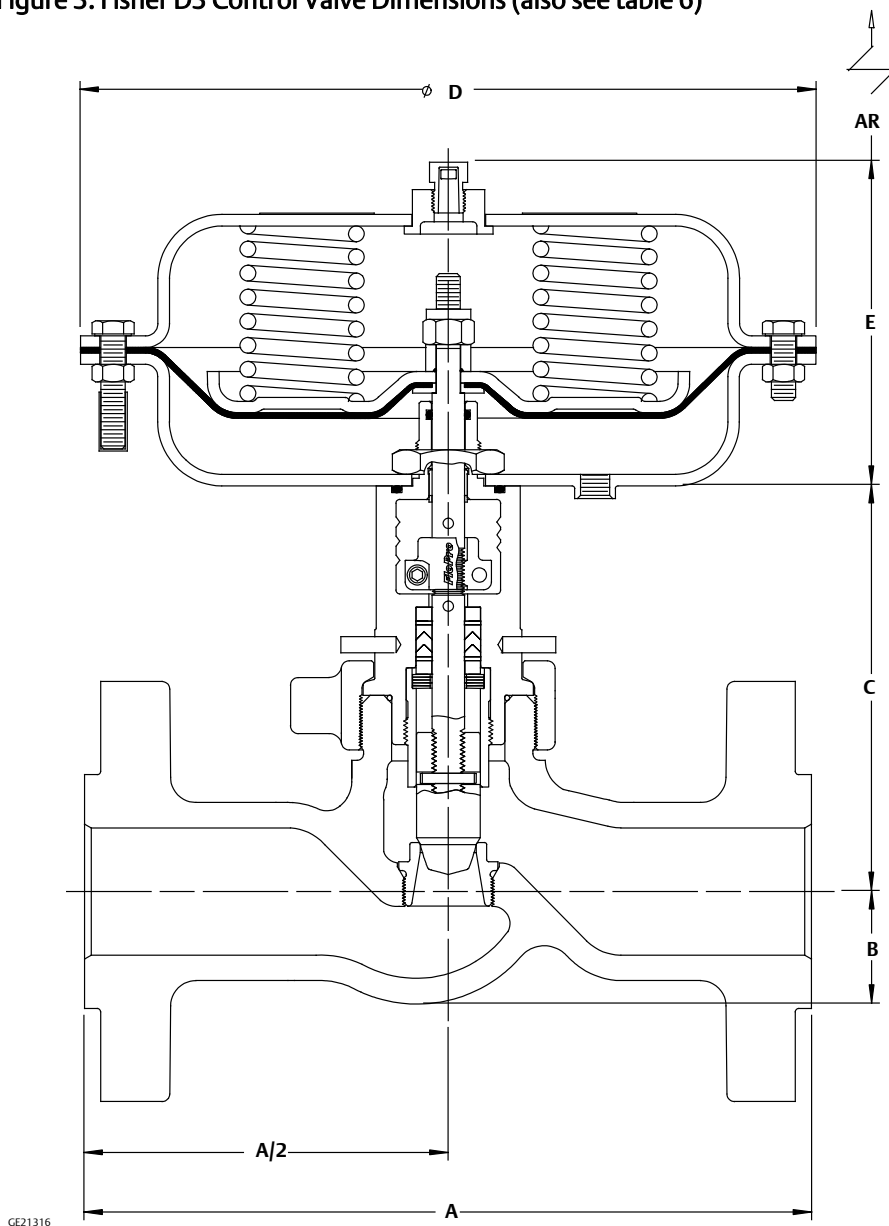
Figure 3. Fisher D3 Control Valve Dimensions (also see table 6)
