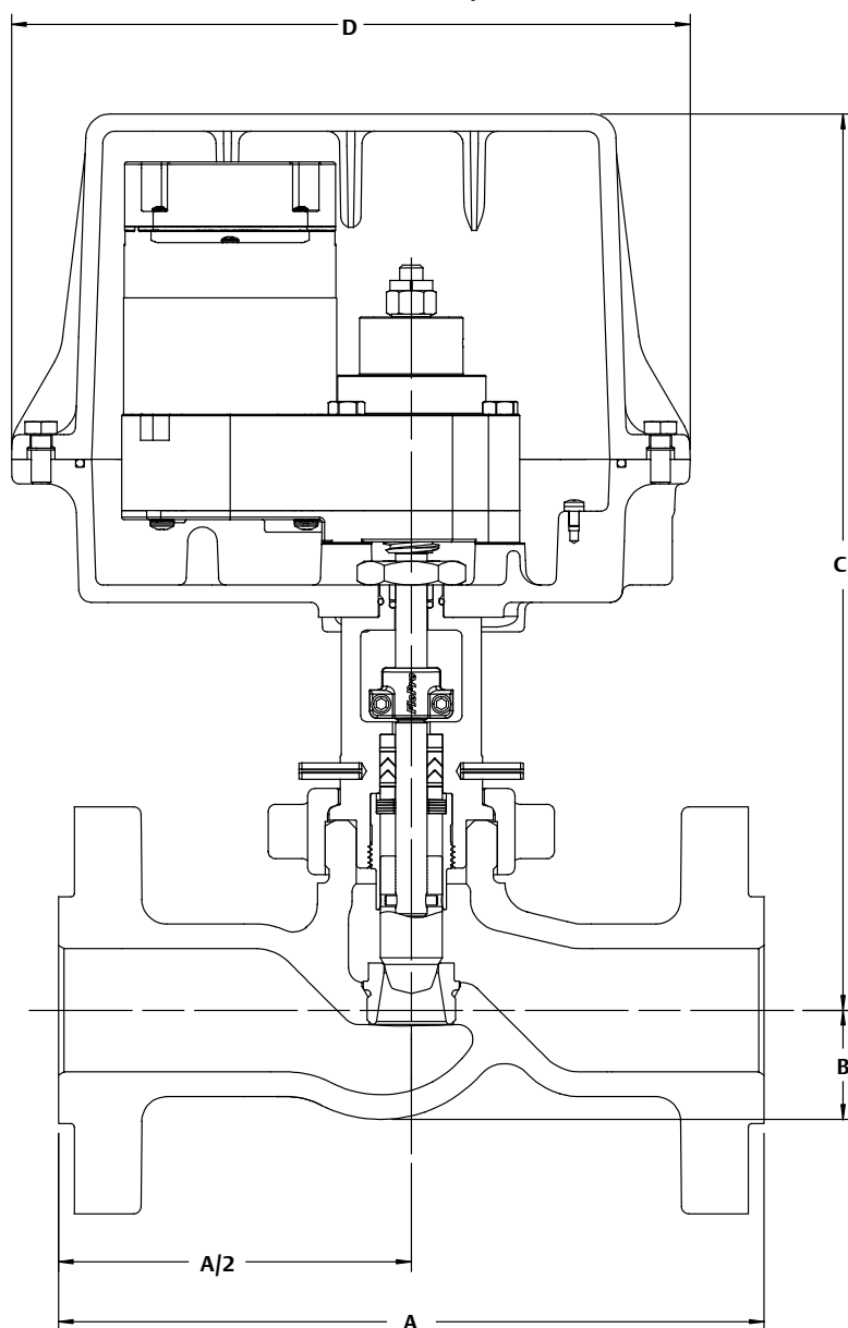
Figure 2. Fisher D3 Control Valve with easy-Drive Electric Actuator and NPS 2 Flanged Valve Body
